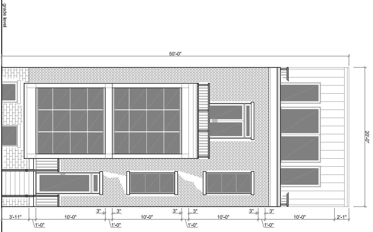
PROPOSED FRONT ELEVATION (10TH STREET) SCALE: 1/4"=1'-0"
